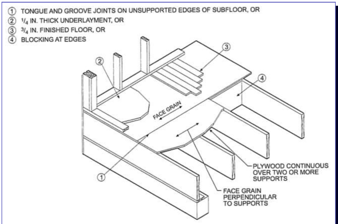
Figure R503.2.2(2) - Combination Subfloor Underlayment Alternatives
